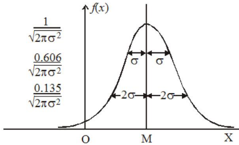
The Gaussian density Function
